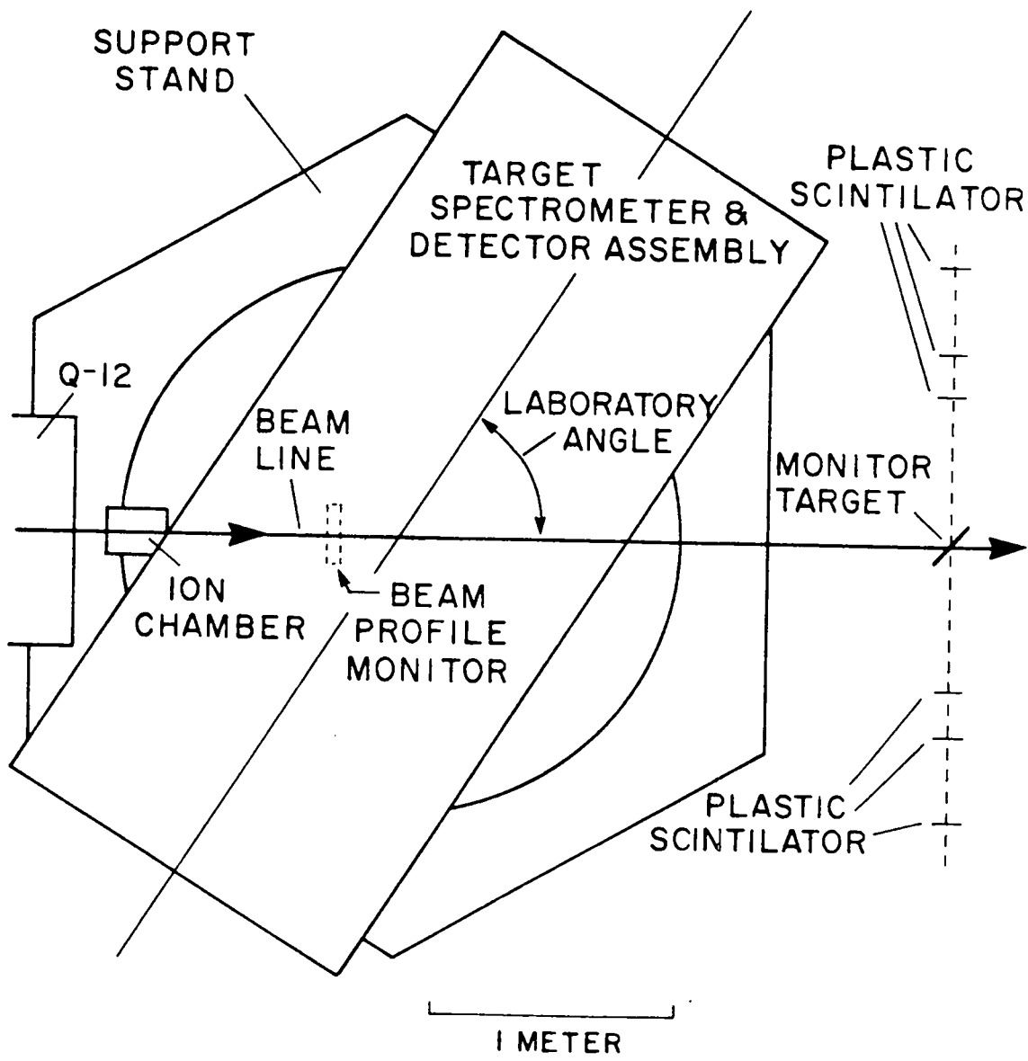
Fig. 1. Plan view of experiment. Q-12 is the last quadrapole magnet of P 3 -west.
