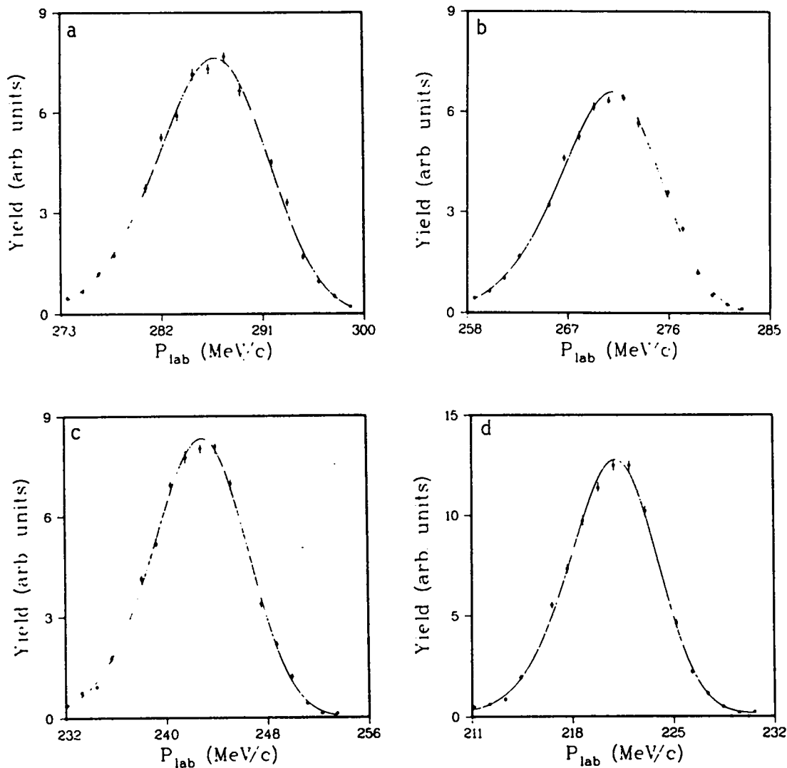
Fig. 16. Sample spectra for \pi^- p \rightarrow \pi^- p at 254 MeV. Spectra are for the laboratory angles a) 70^\circ , b) 80^\circ , c) 100^\circ and d) 120^\circ . The curve was determined by the least squares fitting procedure.
