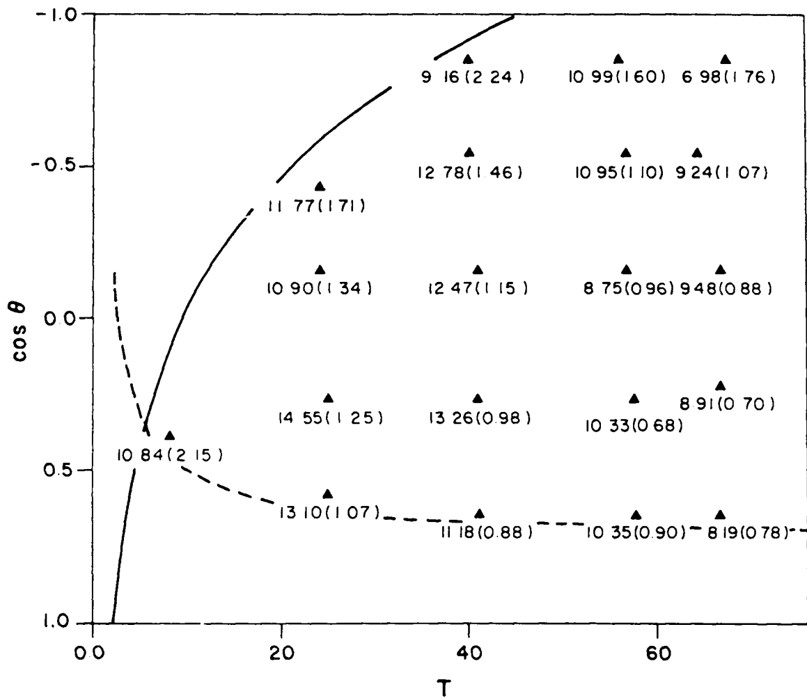
Fig. 33. Values of \langle M \rangle^2 at 292 MeV. The uncertainties are statistical.
